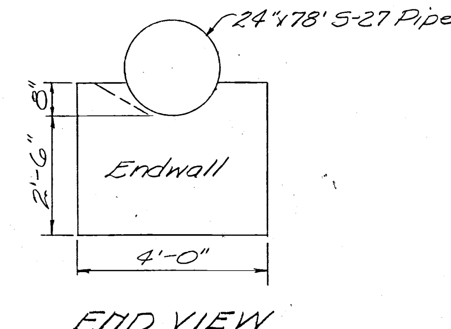
DETAIL OF CONCRETE ENDWALL
