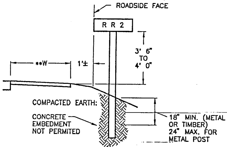
COMBINED DRIVEWAY AND MAIL BOX APPROACH
