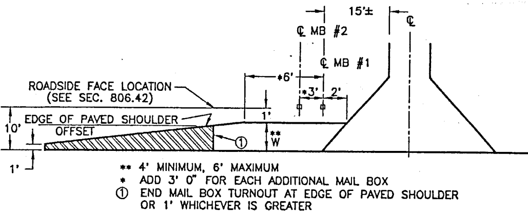
COMBINED DRIVEWAY AND MAIL BOX APPROACH
