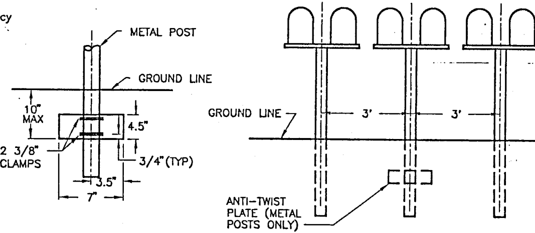
ANTI-TWIST PLATE
