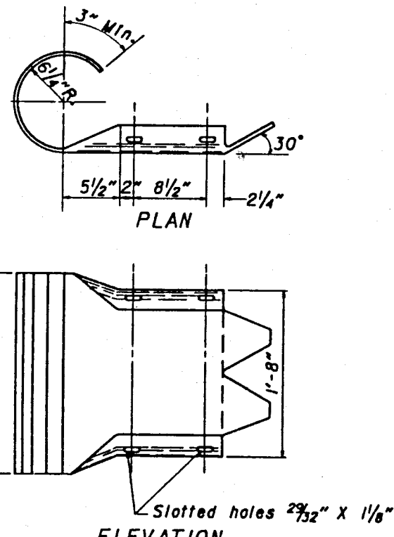
ELEVATION THRIE BEAM ROUNDED END SECTION
