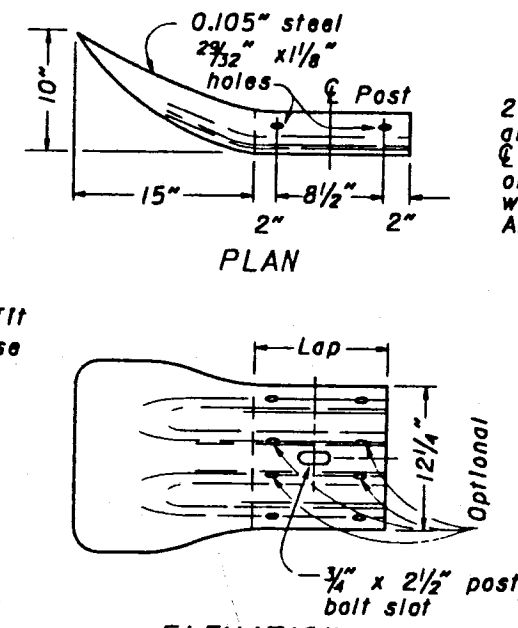
ELEVATION W-BEAM FLARED END SECTION
