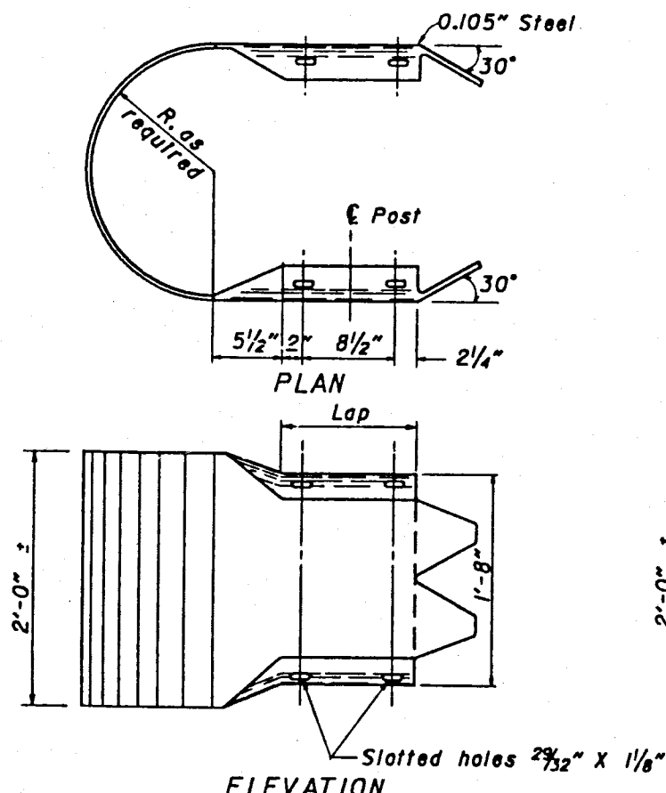
ELEVATION THRIE BEAM BUFFER END SECTION
