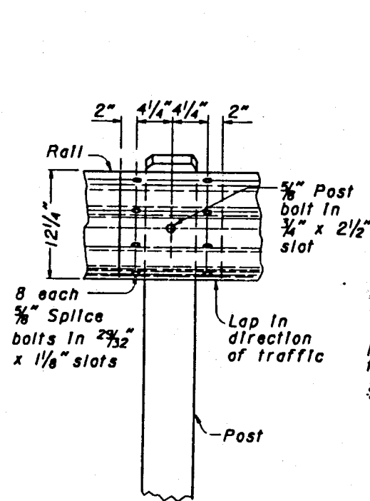
W-BEAM RAIL SPLICE
