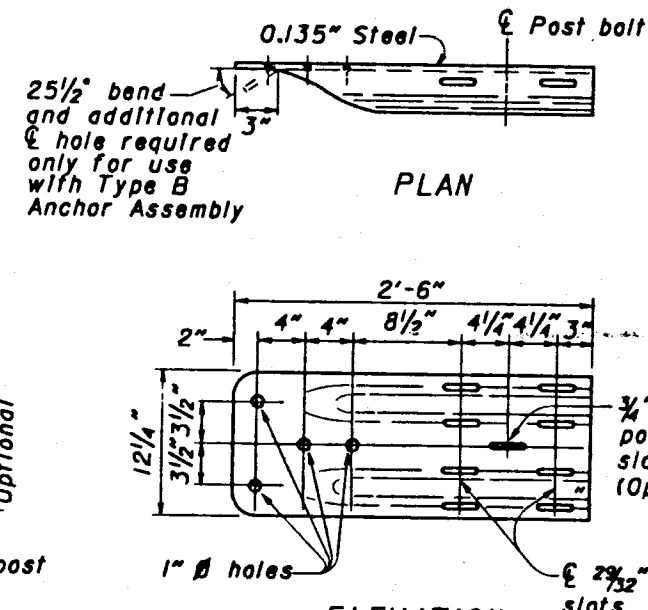
ELEVATION W-BEAM TERMINAL CONNECTOR
