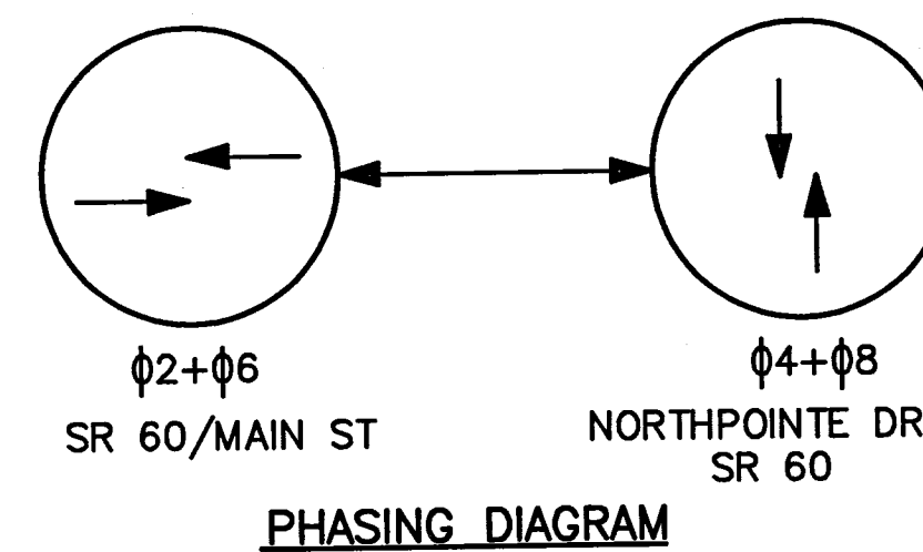
PHASING DIAGRAM
