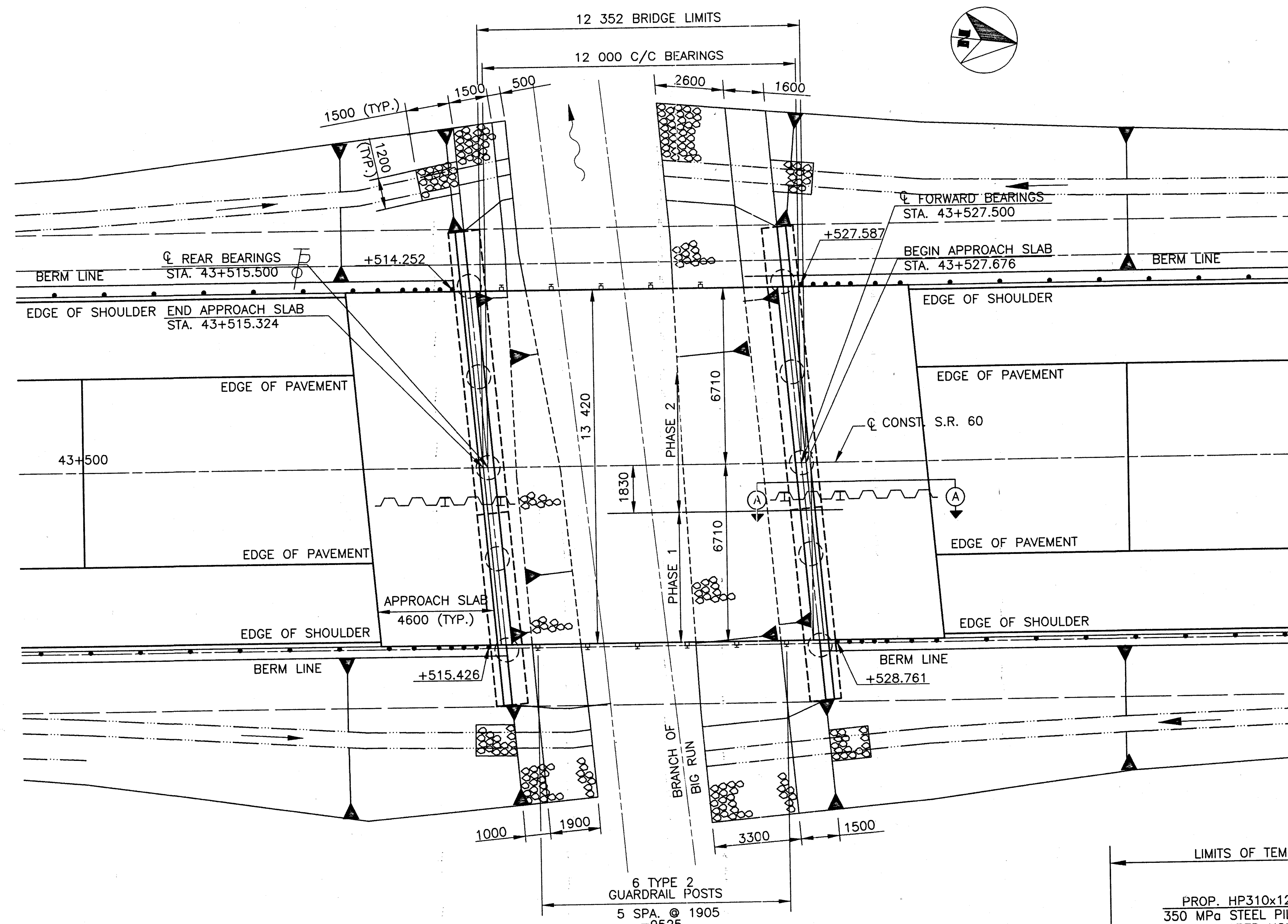
GENERAL PLAN
