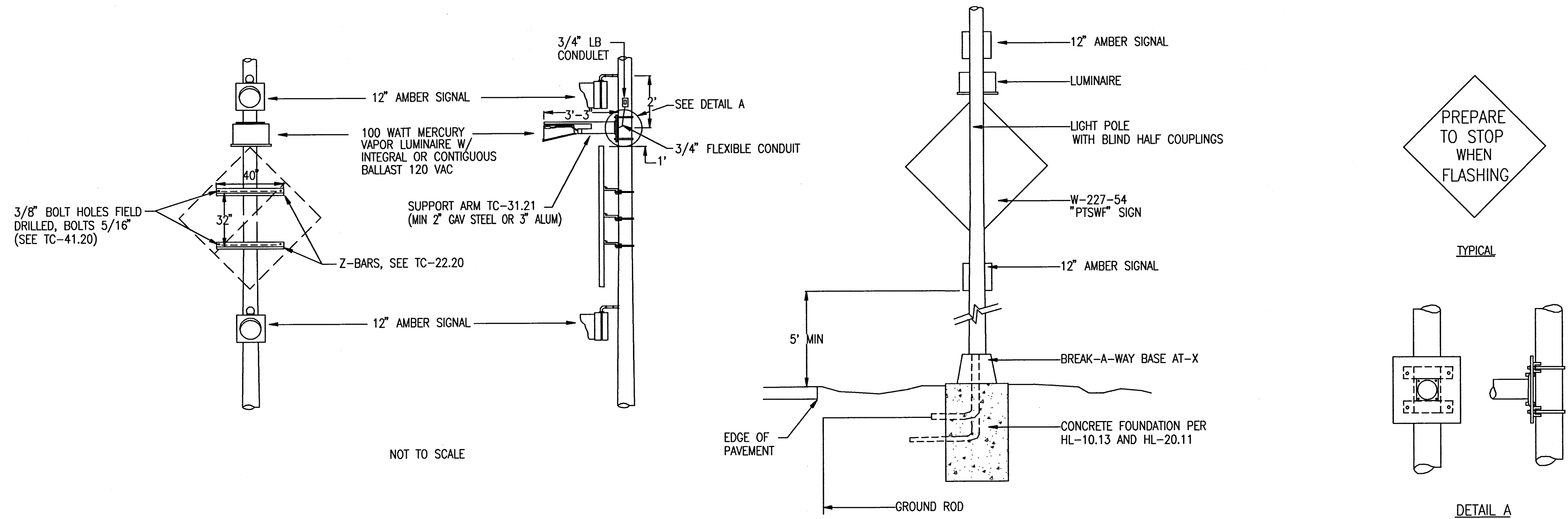
"PREPARE TO STOP WHEN FLASHING" SIGN INSTALLATION DETAIL
