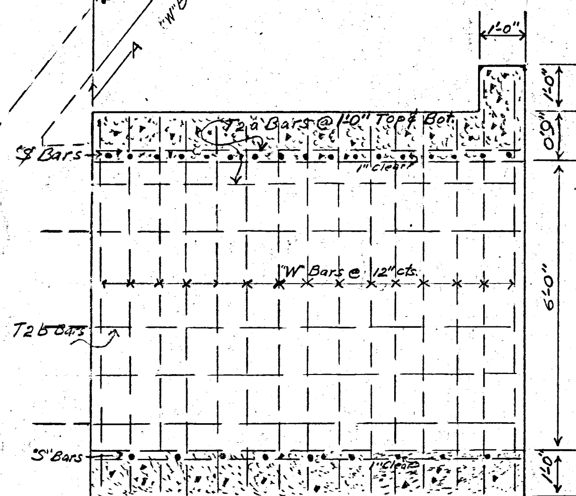
SECTION AA
