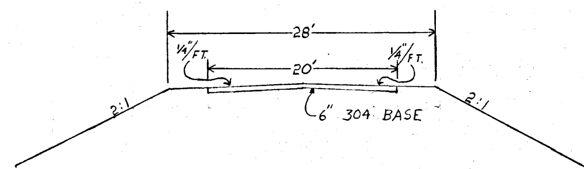
TYPICAL SECTION
