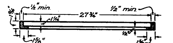
SECTION THROUGH ANGLE FRAME
