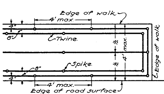
PARKWAY STRIP BETWEEN WALK AND ROAD SURFACE
