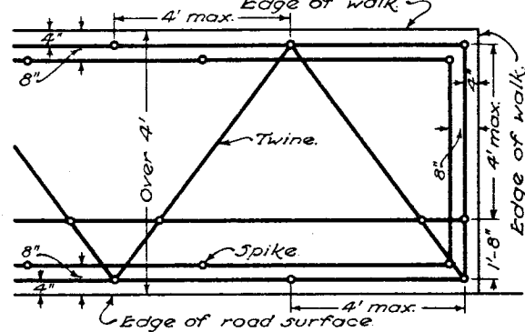
PARKWAY STRIP BETWEEN WALK AND ROAD SURFACE
