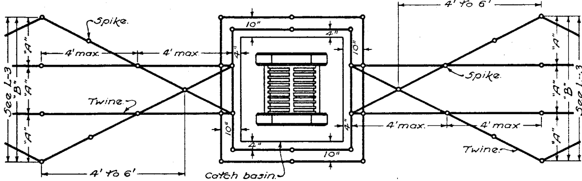
AROUND CATCH BASIN IN SIDE DITCH
