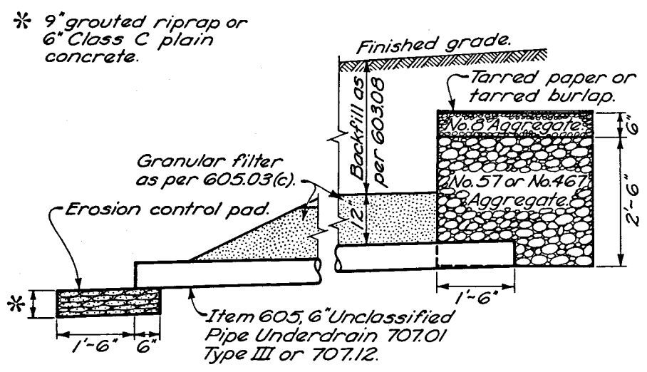
SECTION A-A SPRING DRAIN DETAIL
