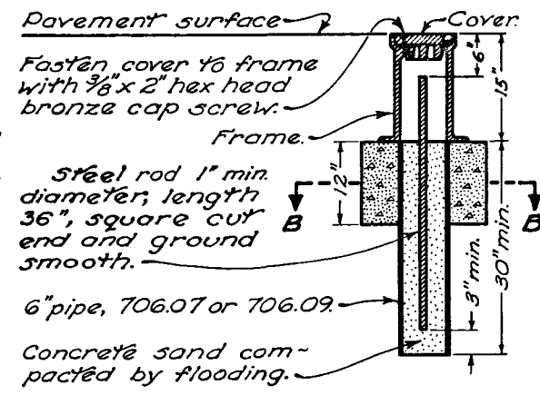
MONUMENT ASSEMBLY SECTION Cost of furnishing and placing monument box, steel rod, class C concrete, concrete sand and pipe included in price bid for 604 Monument Assembly.
