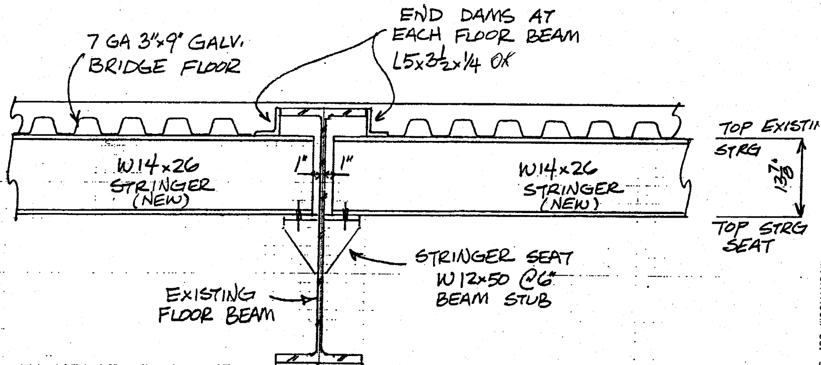
DETAIL AT FLOOR BEAM
