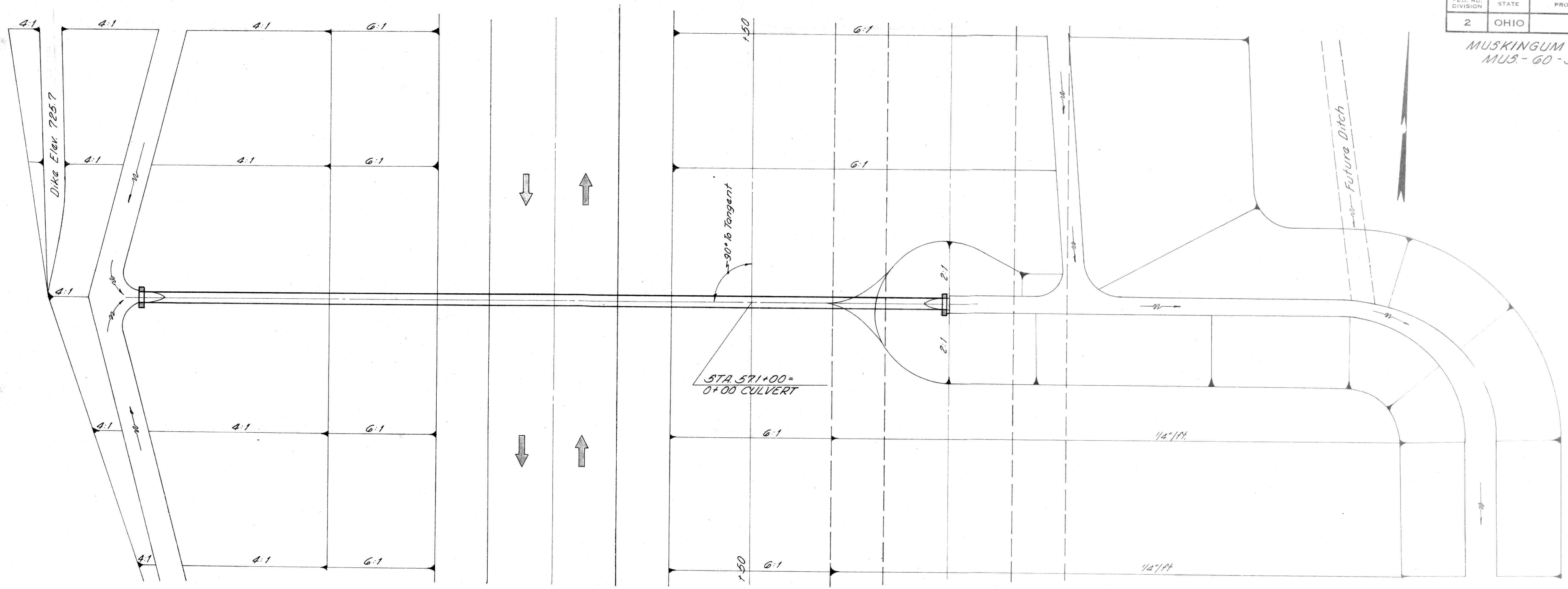
PLAN
