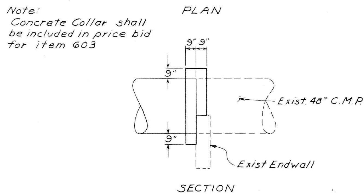
CONCRETE COLLAR DETAIL - 'A'
