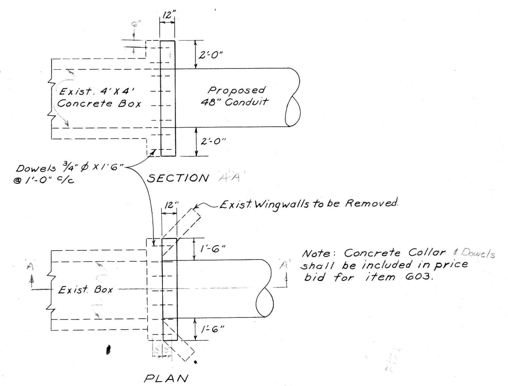
CONCRETE COLLAR DETAIL - 'B'
