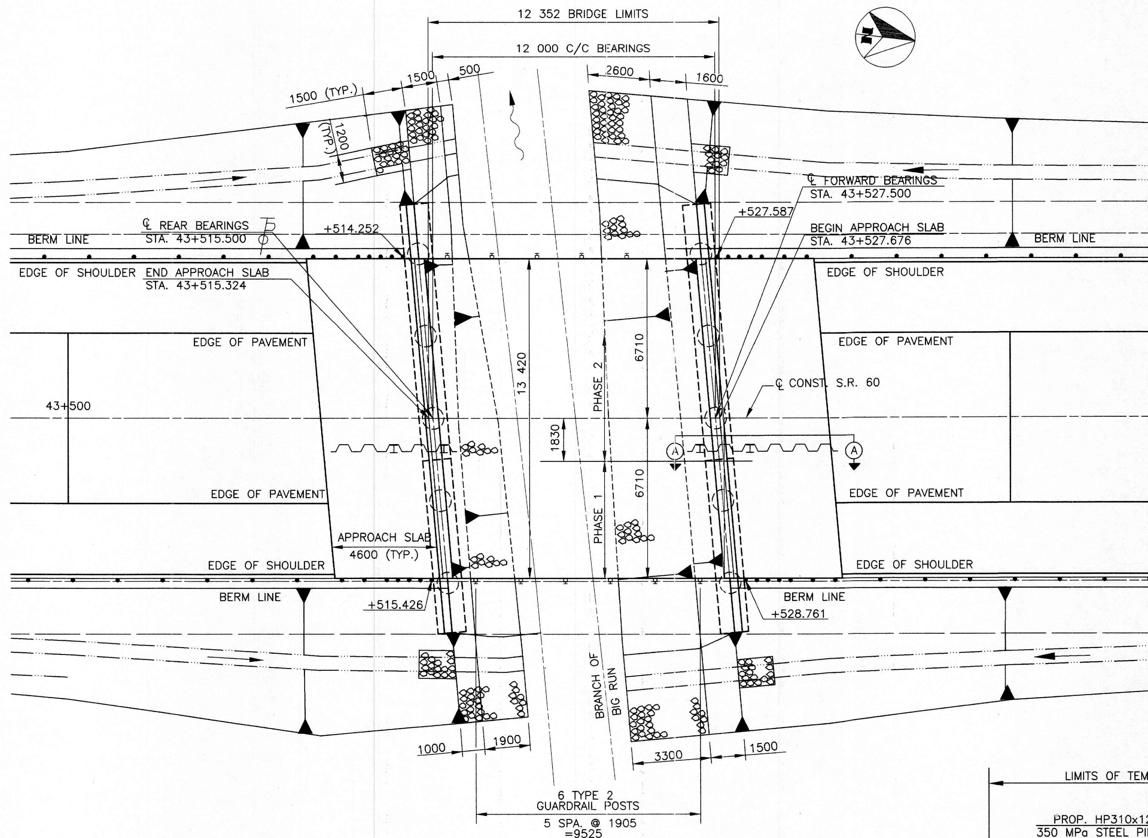
GENERAL PLAN
