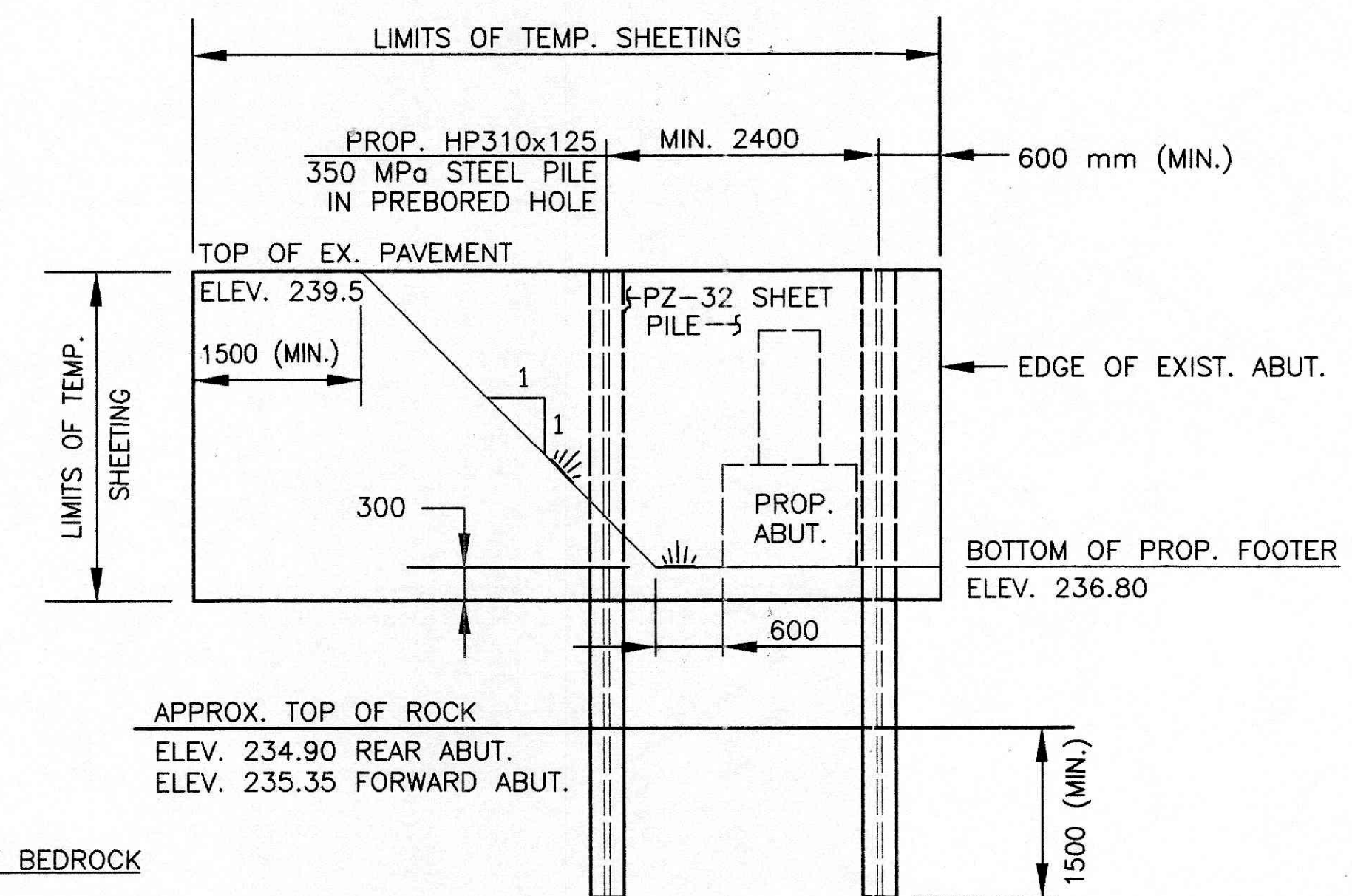
SECTION A-A TYPICAL TEMPORARY SHEETING LIMITS
