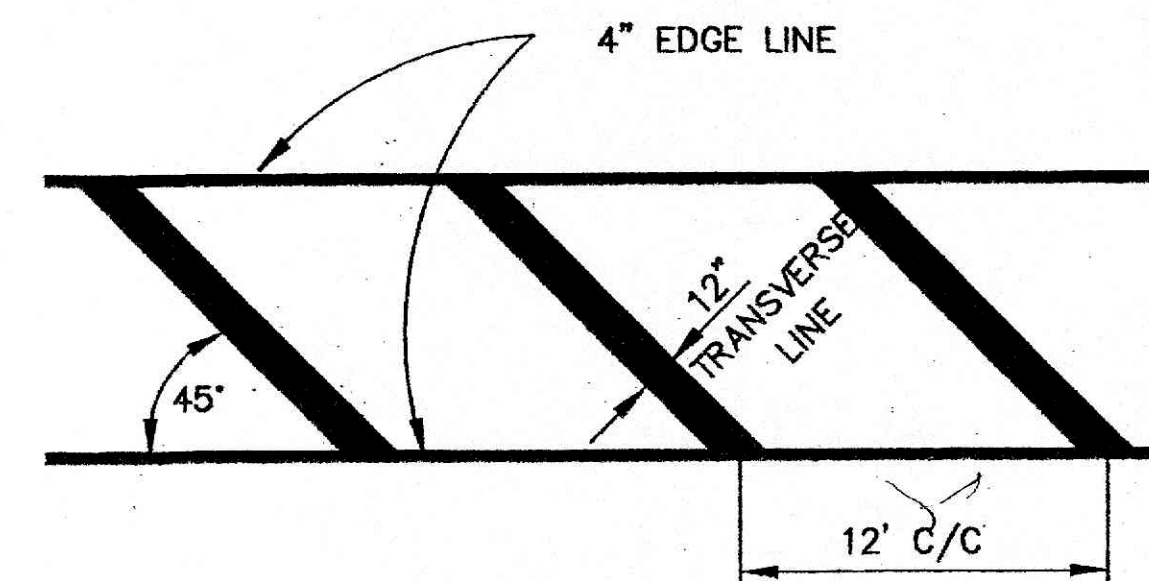
TYPICAL ISLAND MARKING DETAIL
