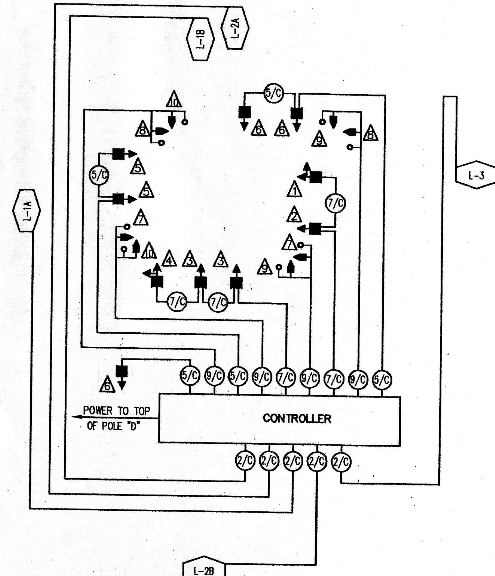
WIRING DIAGRAM
