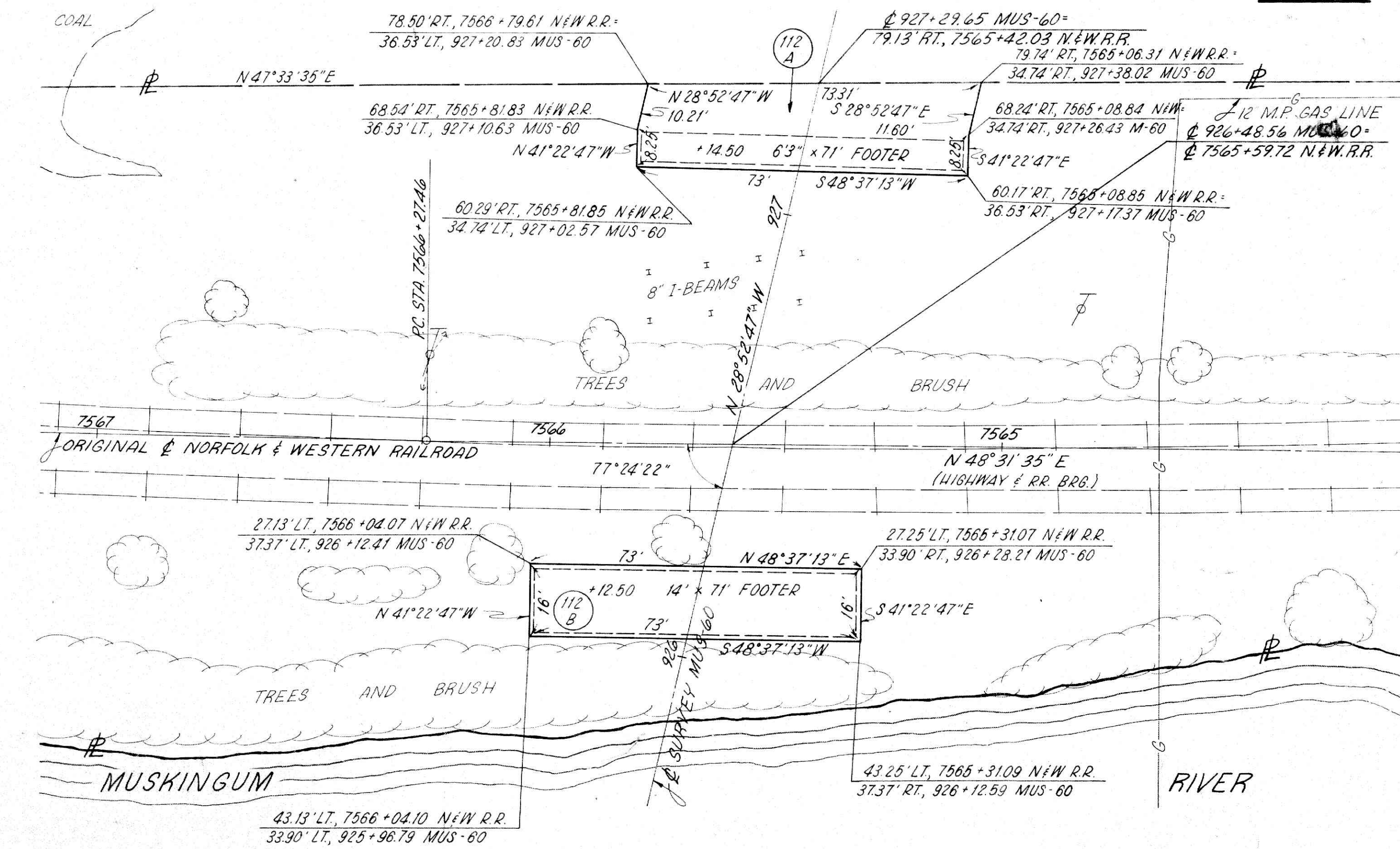
HIGHWAY OCCUPATIONAL EASEMENT 1"=20'
