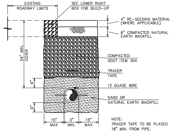
TYP. PIPE TRENCH DETAIL (PARALLEL TO EXISTING ROADWAYS) FOR TOWNSHIP ROADS
