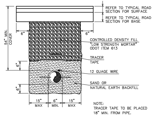
TYP. PIPE TRENCH DETAIL (PAVEMENT AREAS) FOR COUNTY ROADS AND/OR STATE ROUTES
