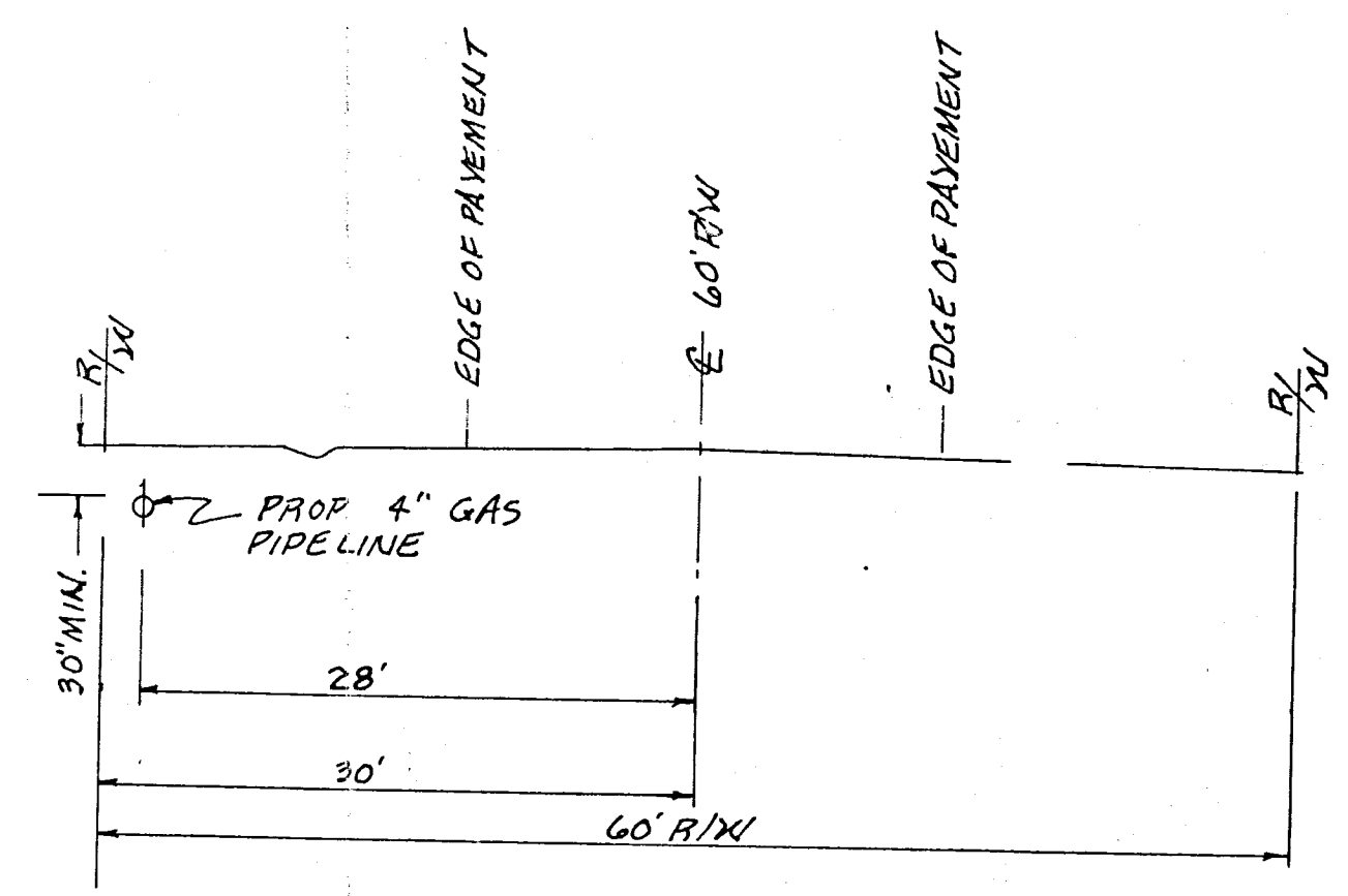
CROSS SECTION @ 60' R/W SCALE 1" = 10'
