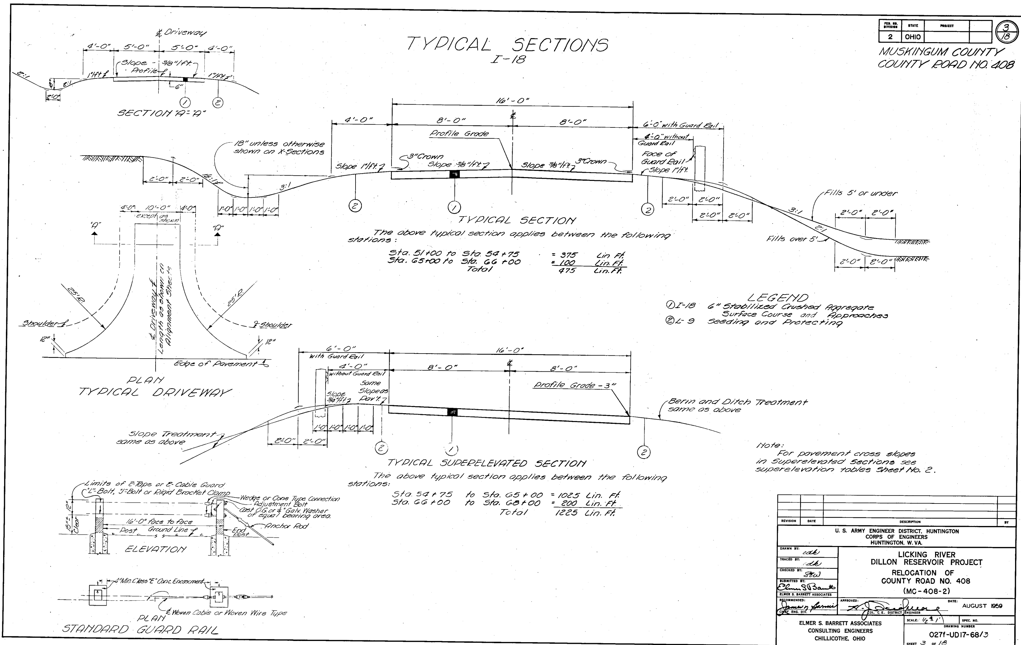
TYPICAL SECTIONS & DETAILS
