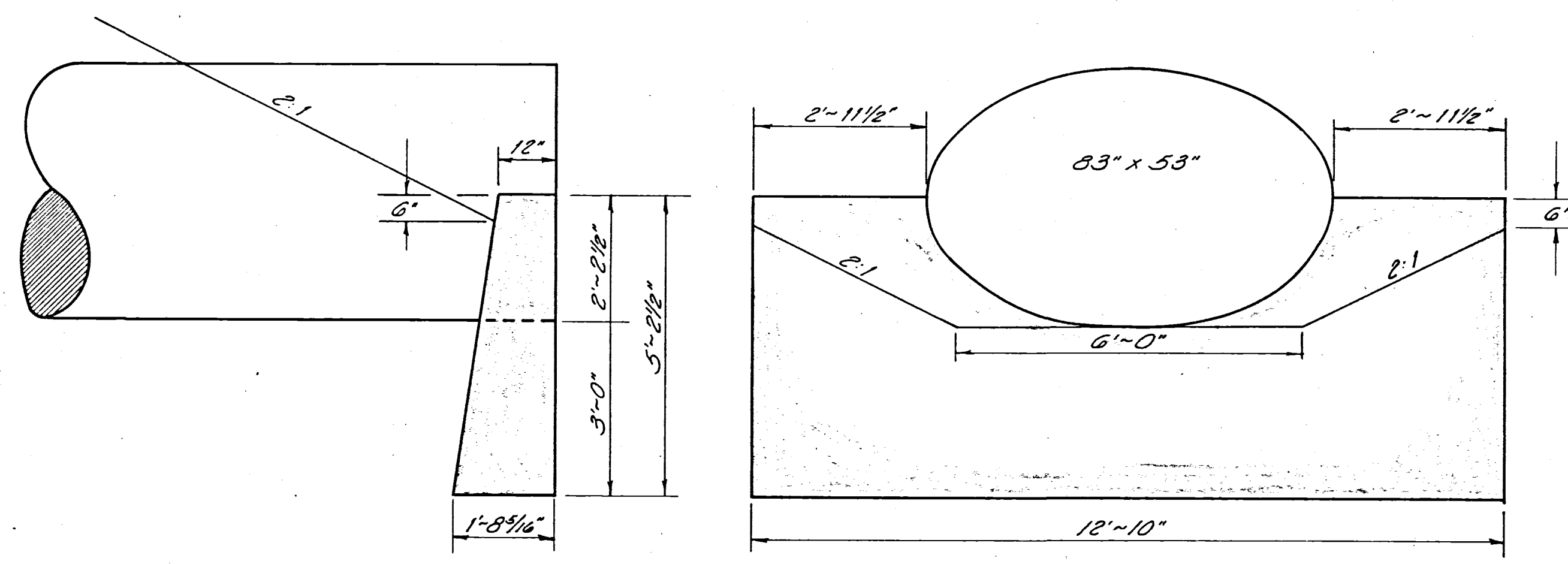
DETAIL SP53 ENDWALL Scale: 1/2" = 1'-0"
