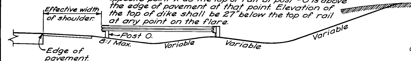
SECTION A-A CUT TO FILL
