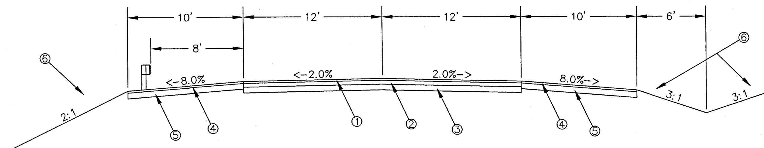
TYPICAL ROAD SECTION SCALE: 1" = 5'
