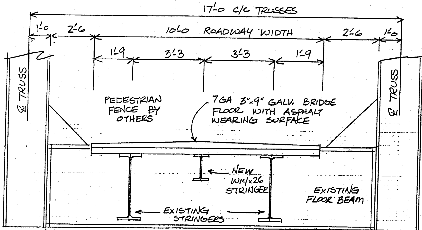
BRIDGE SECTION VIEW
