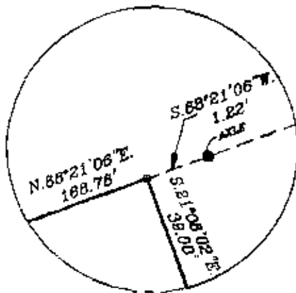
CORNER DETAIL
