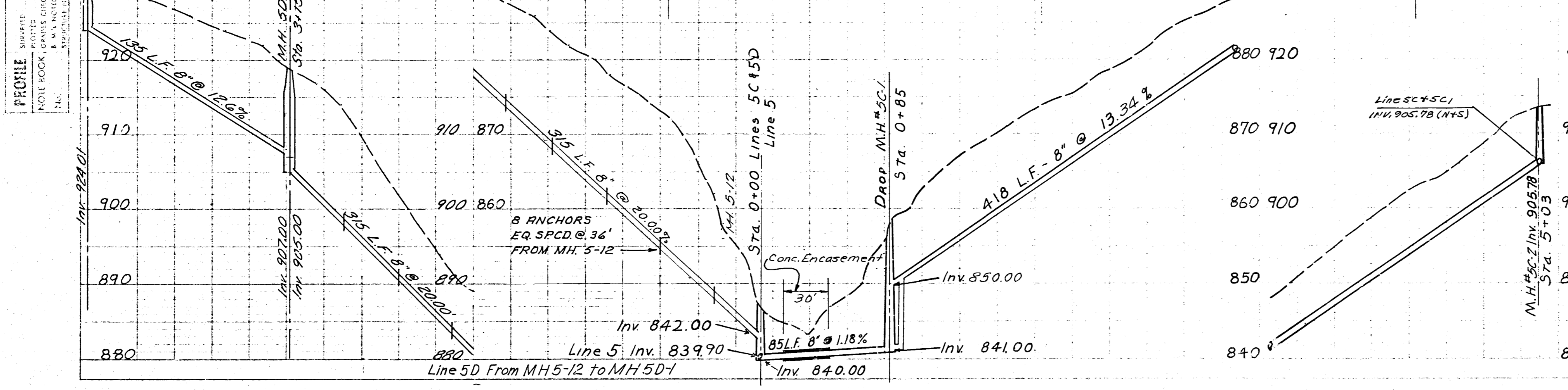
SEWER LINE 5-C M.H.#5C-12-M.H.#5C-2
