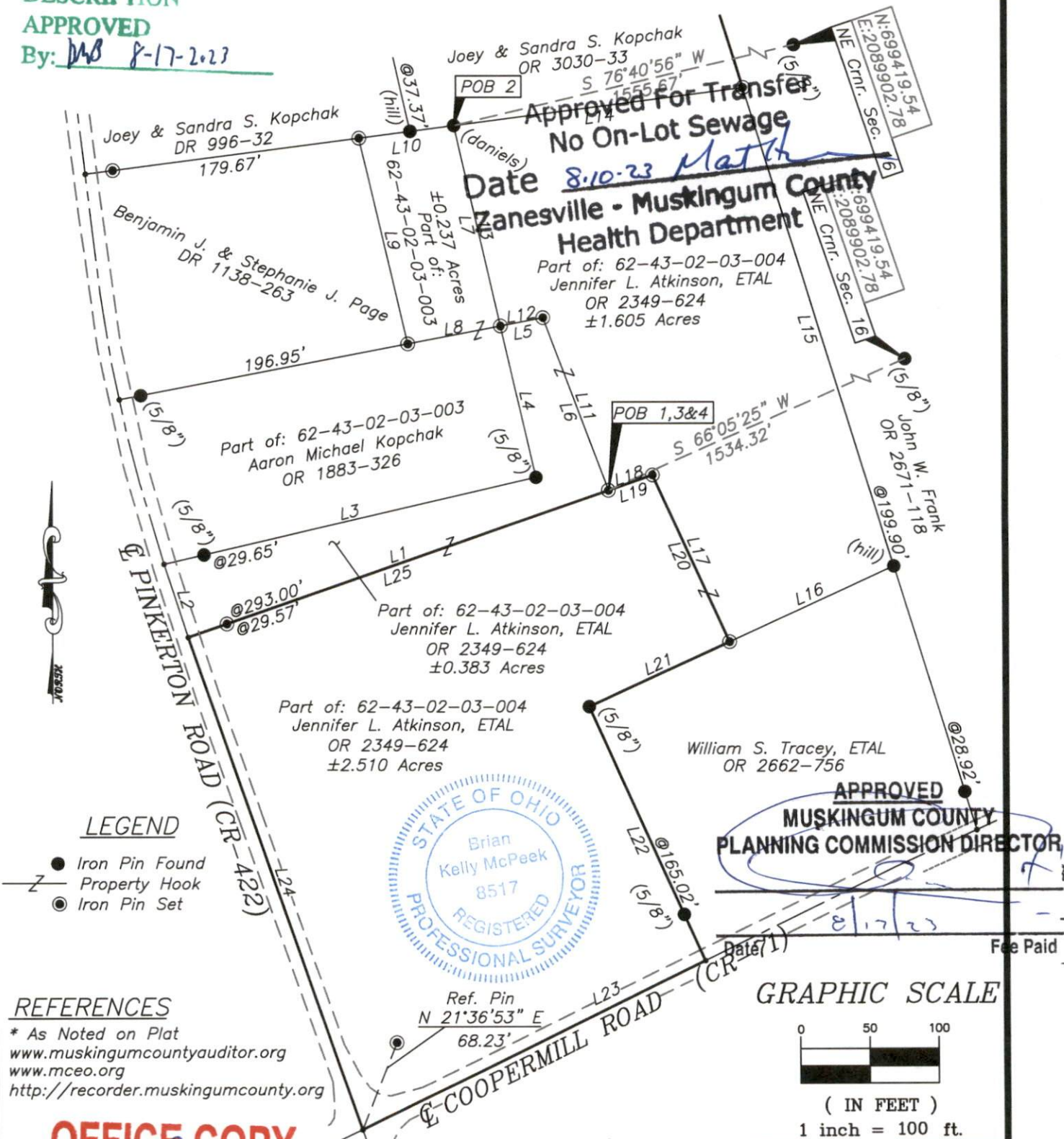
LINE BEARING DISTANCE LINE BEARING DISTANCE L1 S 70°54'21" W 322.57' L13 N 12°58'29" W 148.30' L2 N 18°09'30" W 55.45' L14 N 82°33'37" E 211.04' L3 N 76°59'22" E 276.62' L15 S 17°18'01" E 361.99' L4 N 13°00'02" W 112.44' L16 S 65°19'34" W 130.47' L5 N 79°07'03" E 31.32' L17 N 24°39'58" W 132.38' L6 S 20°40'17" E 133.51' L18 S 70°54'21" W 33.79' L7 S 12°58'29" E 148.30' L19 N 70°54'21" E 33.79' L8 S 79°07'03" W 68.46' L20 S 24°39'58" E 132.38' L9 N 13°13'51" W 152.46' L21 S 65°19'34" W 111.95' L10 N 82°31'49" E 69.42' L22 S 24°24'08" E 201.63' L11 N 20°40'17" W 133.51' L23 S 63°54'26" W 277.44' L12 S 79°07'03" W 31.32' L24 N 19°15'28" W 377.21' L25 N 70°54'21" E 322.57'
