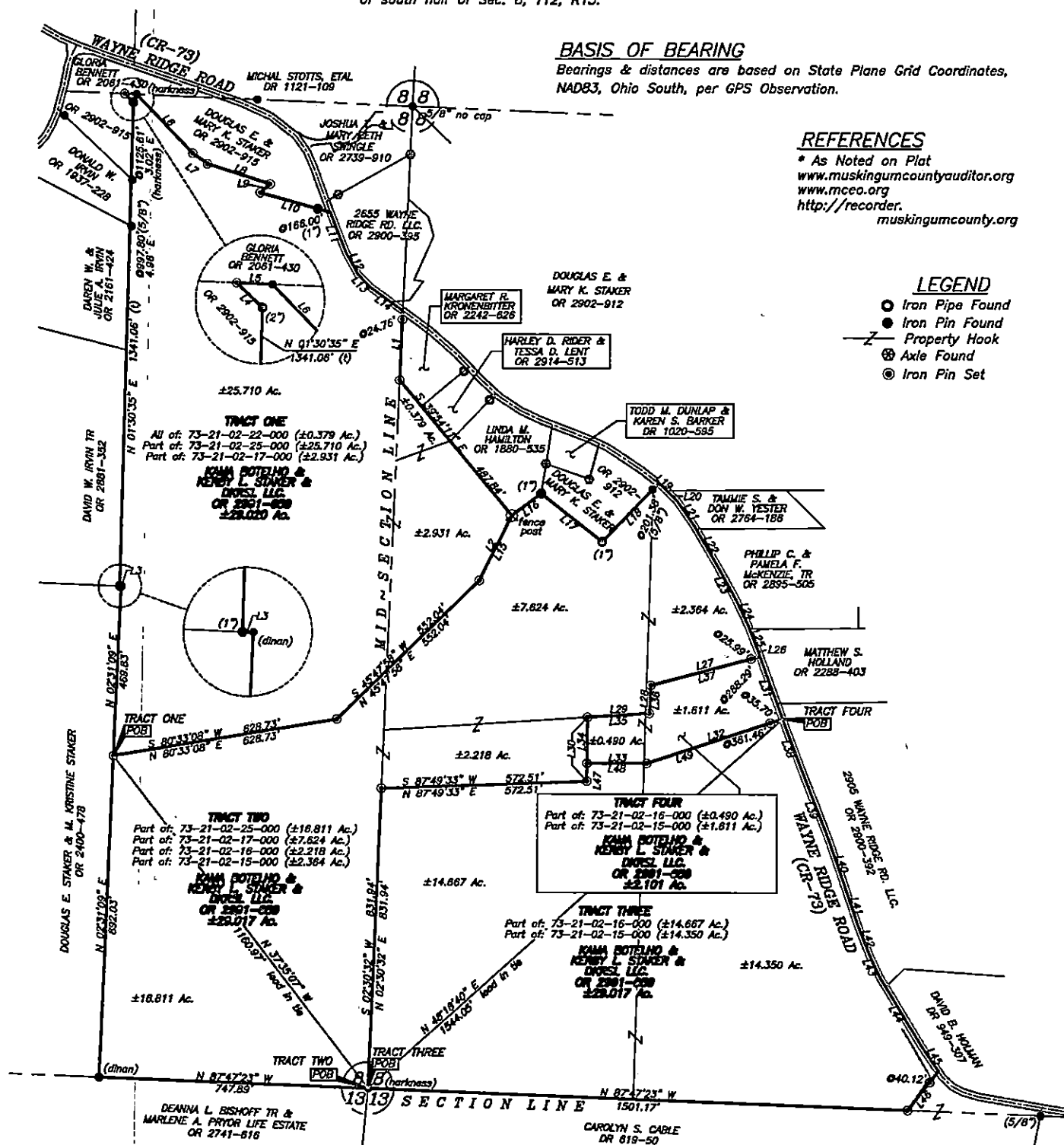
LINE BEARING 1954/2002 L25 S 21°29'29" E 77.88 L1 S 02°30'32" W 151.41 L26 S 15°31'59" E 127.71 L2 S 26°50'32" W 201.72 L27 S 75°10'24" W 314.27 L3 N 47°45'18" W 3.77 L28 S 02°53'23" W 77.88 L4 N 45°57'26" W 33.03 L29 S 85°18'38" W 172.81 L5 N 07°41'44" E 32.92 L30 S 00°32'48" W 177.58 L6 S 43°52'44" E 223.88 L31 S 19°54'49" E 183.97 L7 S 61°11'36" E 33.70 L32 N 71°50'41" E 339.16 L8 S 26°19'39" E 182.70 L33 N 00°32'18" W 166.07 L9 S 49°50'42" W 58.16 L34 N 00°32'18" W 127.81 L10 S 74°34'06" E 202.18 L35 N 88°15'39" E 77.88 L11 S 21°16'52" E 118.25 L36 N 02°53'23" E 314.27 L12 S 29°27'08" E 70.45 L37 N 75°10'24" E 168.31 L13 S 44°17'44" E 50.57 L38 S 20°32'14" E 195.92 L14 S 43°53'56" E 110.11 L39 S 21°07'36" E 136.50 L15 N 20°00'32" E 212.62 L40 S 18°53'09" E 101.69 L16 N 53°03'03" E 101.80 L41 S 18°05'05" E 65.72 L17 S 51°57'03" E 215.65 L42 S 21°12'59" E 65.72 L18 N 44°08'04" E 225.27 L43 S 25°30'44" E 222.63 L19 S 52°09'33" E 16.25 L44 S 31°12'42" E 84.17 L20 S 45°24'24" E 54.47 L45 S 34°04'30" E 138.51 L21 S 37°13'16" E 63.16 L46 S 38°07'13" W 49.88 L22 S 30°13'27" E 110.25 L47 N 00°32'48" W 167.58 L23 S 26°07'52" E 100.56 L48 N 21°30'41" E 307.16 L24 S 24°59'31" E 83.83
